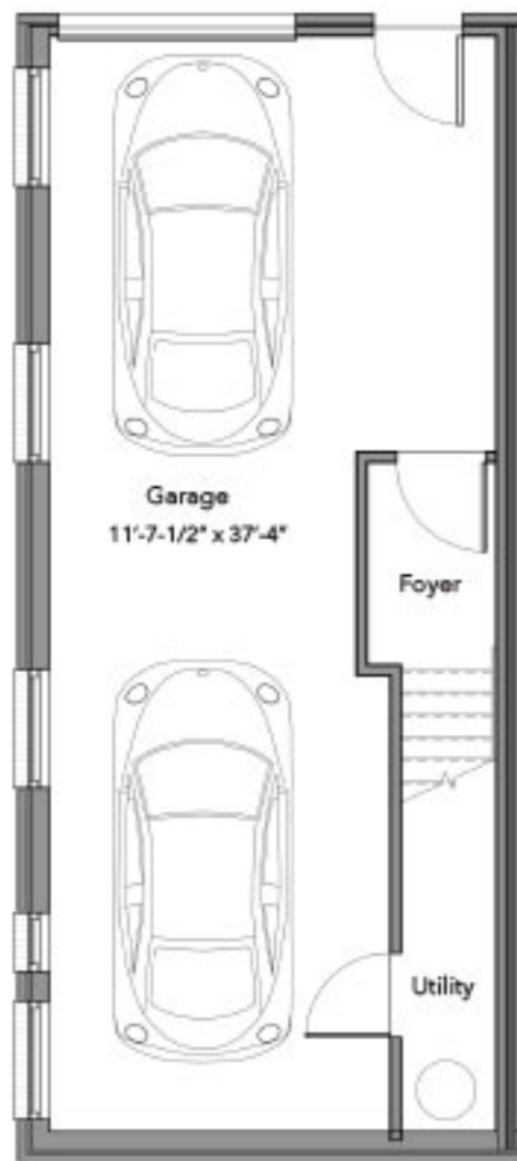
First Level
