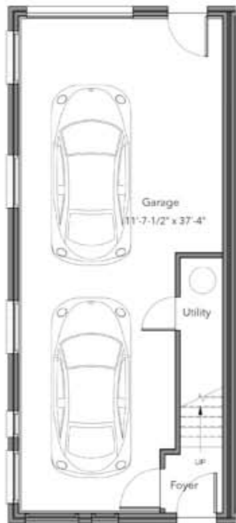
First Level
